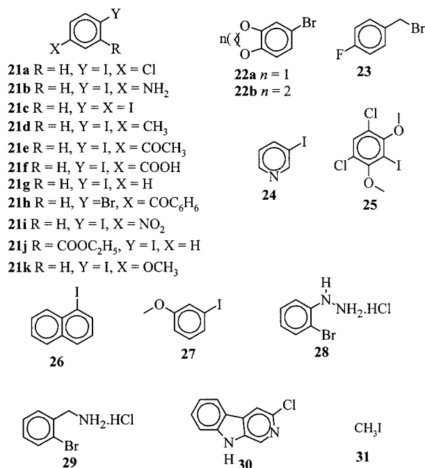
Figure 2. Halides
