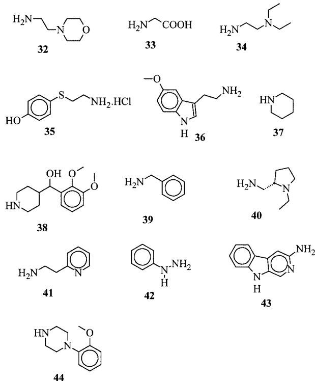
Figure 3. Amines
